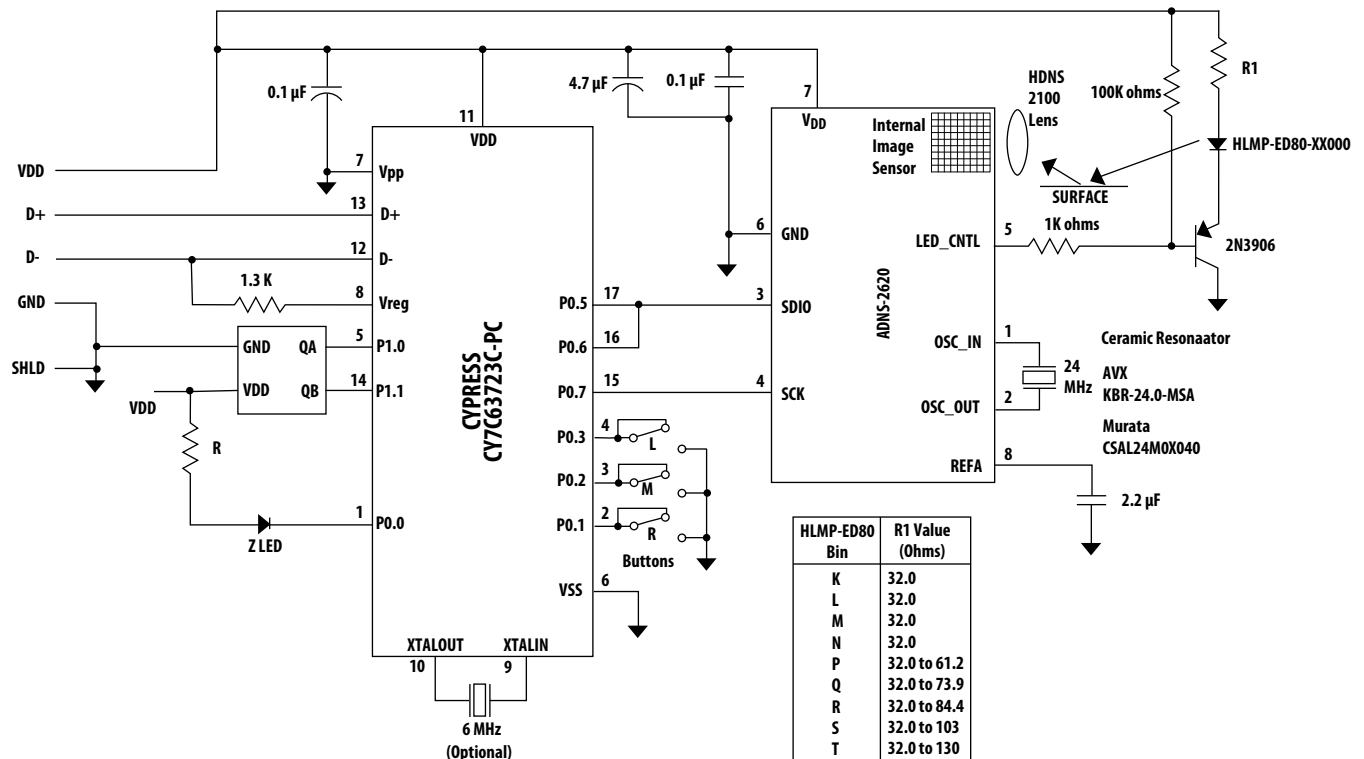
Figure 3. Circuit block diagram for ADNK-2623 designer's kit optical mouse using the Avago ADNS-2620 optical mouse sensor and Cypress CY7C63723C-PC CoRe USB Controller.
